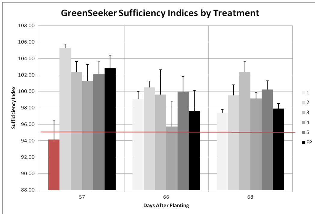
Figure 3.11. GreenSeeker™ treatment nitrogen sufficiency indices over time in Lenoir City, TN.
