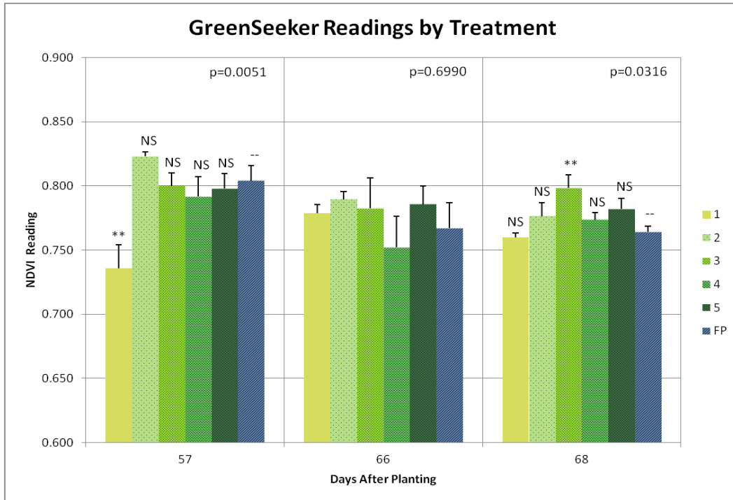
Figure 3.10. Treatment effects on GreenSeeker™ values over time in Lenoir City, TN.
